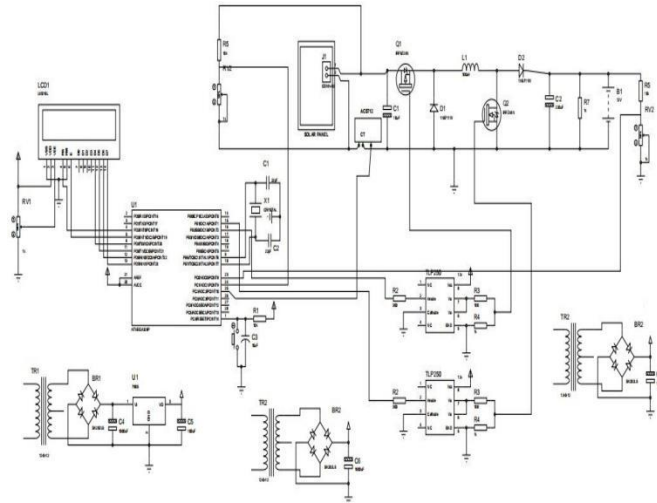
Fig. 2. Circuit Diagram of the Charging Section of Photovoltaic Panel Based Water Pumping System
